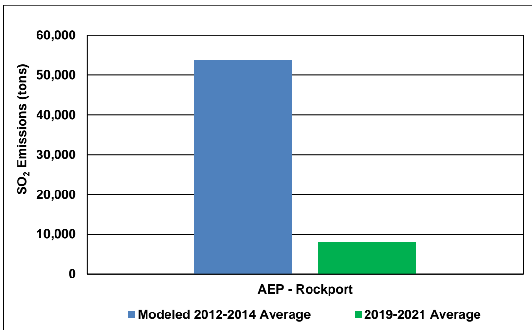
Chart 3: SO 2 Emissions for Spencer County Area
