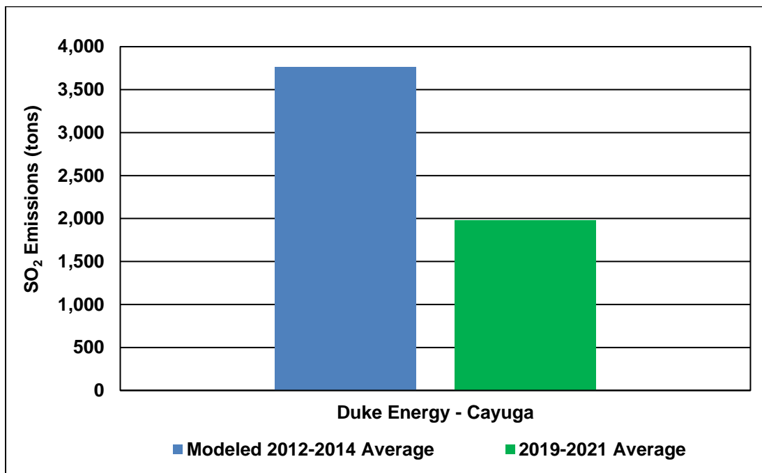
Chart 6: SO 2 Emissions for the Vermillion County Area
