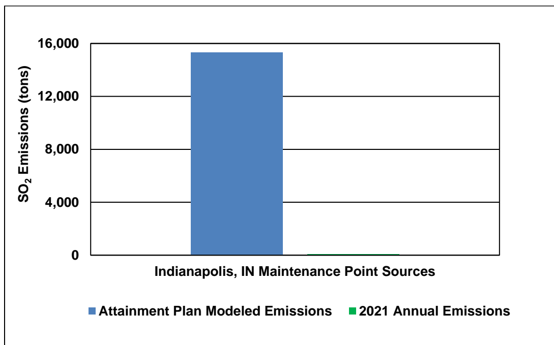
Chart 2: SO 2 Emissions for the Indianapolis, IN Maintenance Area
