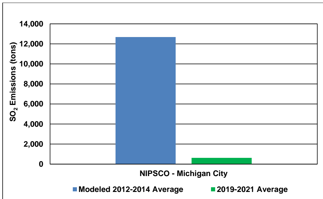
Chart 4: SO 2 Emissions for the La Porte County Area
