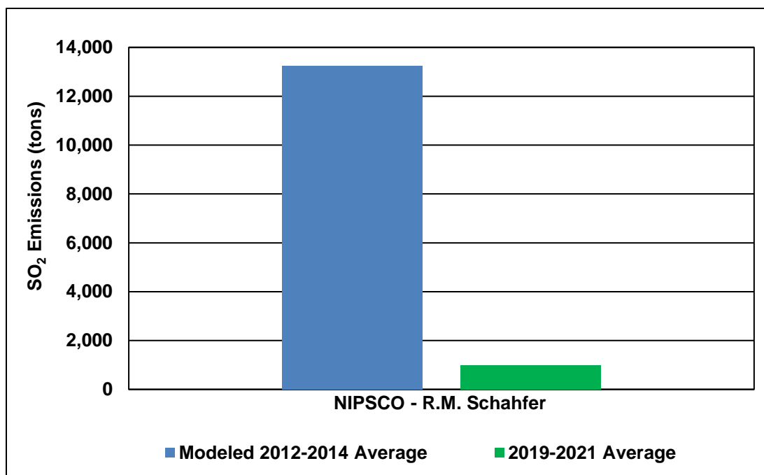
Chart 5: SO 2 Emissions for the Jasper County Area
