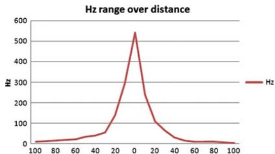
Figure 18.3.3 Noise in Hz 100 m from a leak on 500 mm cast iron pipe at 41 m pressure.
